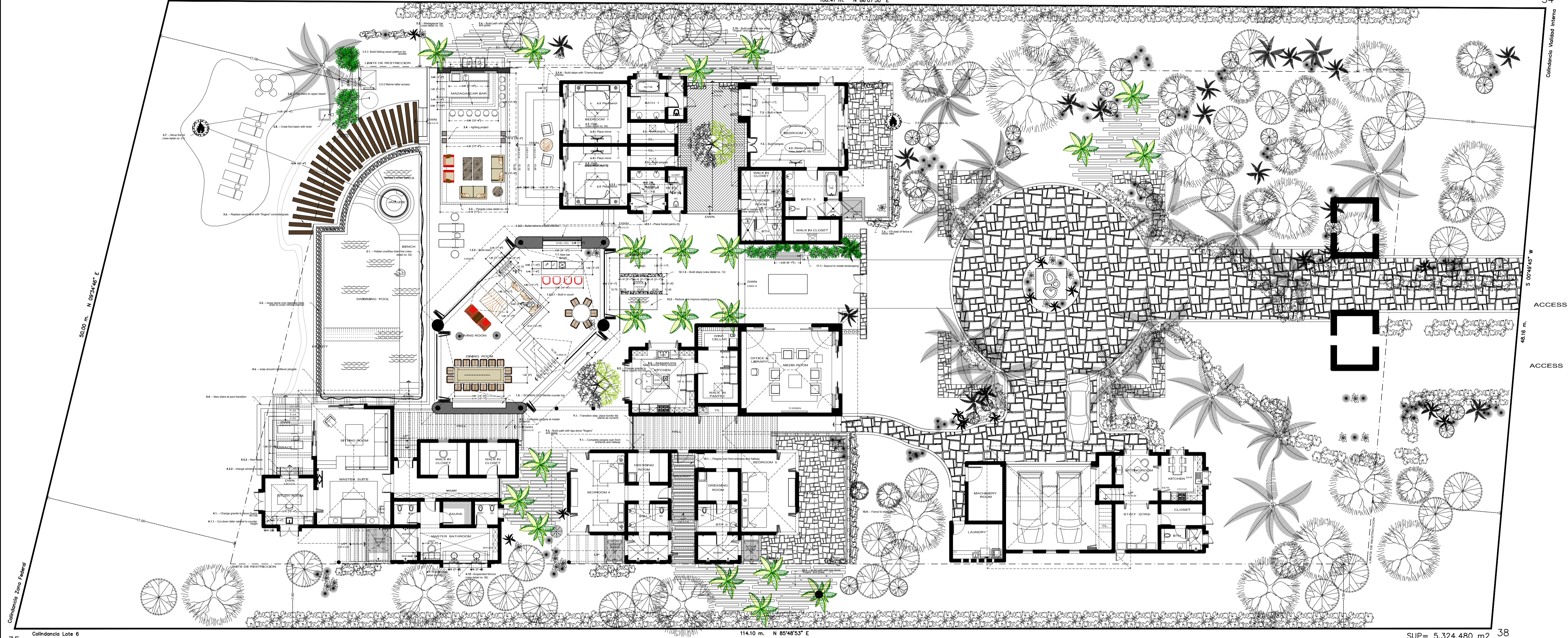
MAIN LEVEL FLOOR PLAN
